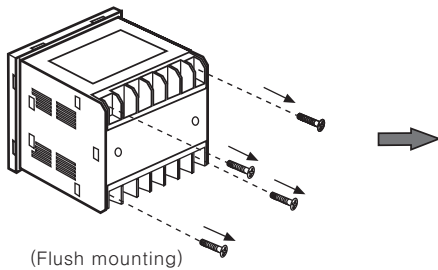
① Unscrew 4 bolts from terminal block.
