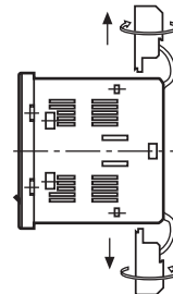
③ Assemble terminal block to case by using the 4 bolts.
