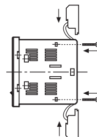
③ Assemble terminal block to case by using the 4 bolts.
